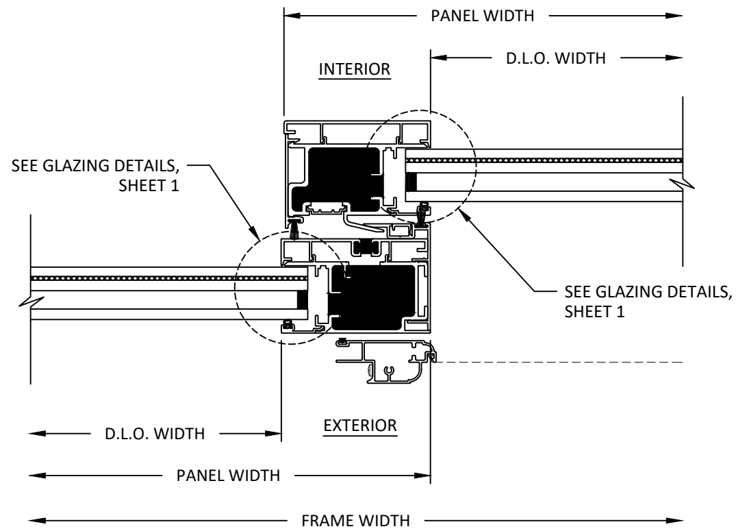
D 5 HORIZONTAL SECTION INTERLOCK
