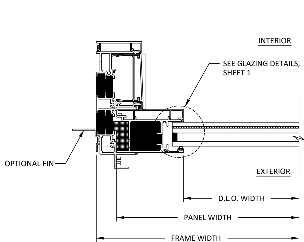
C 5 HORIZONTAL SECTION FIXED JAMB
