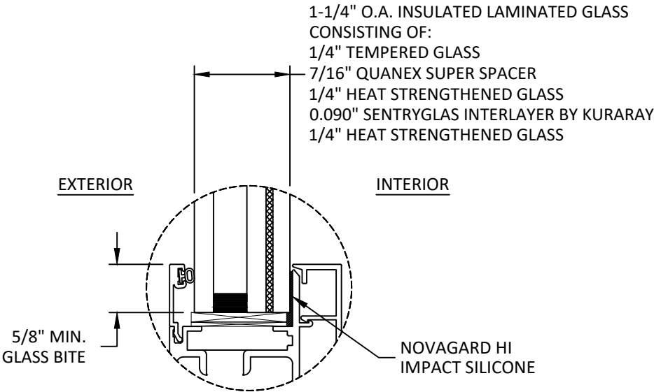
GLAZING DETAIL 1
