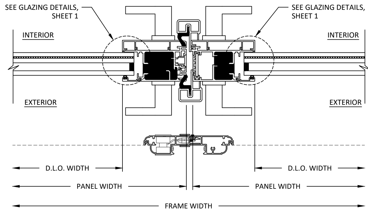
E 5 HORIZONTAL SECTION MEETING STILE
