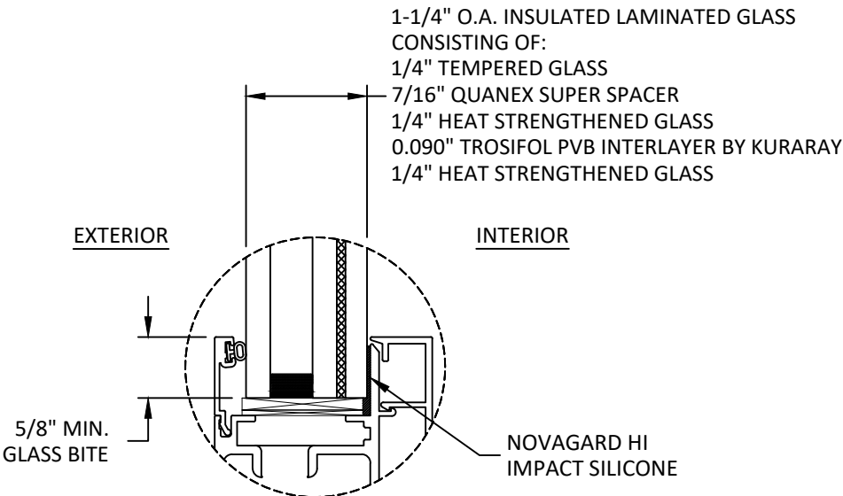
GLAZING DETAIL 2
